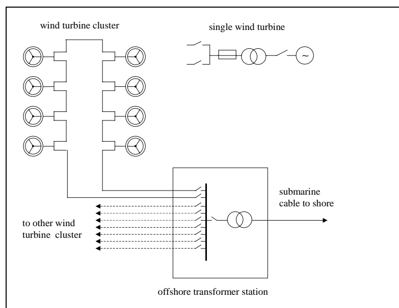
Fig. 3.5: Connection of the wind turbines by a ringed network.
