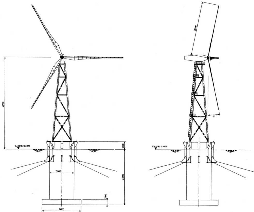
Fig. 3.4 Buoy type support structure [18].
