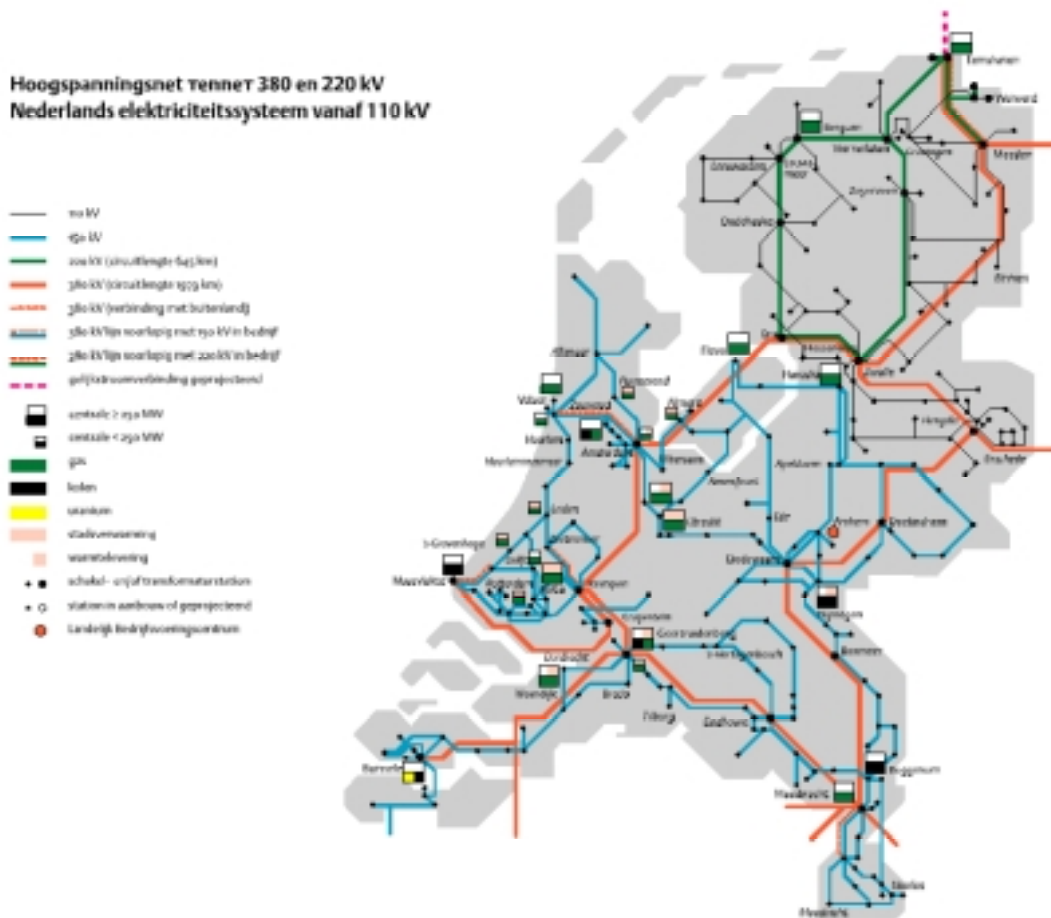
Fig. 3.9: High-voltage grid of the Netherlands [www.Tennet.de].
