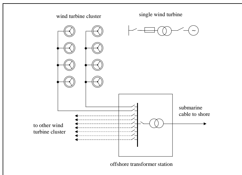
Fig. 3.6 Connection of the wind turbines by a radial network.
